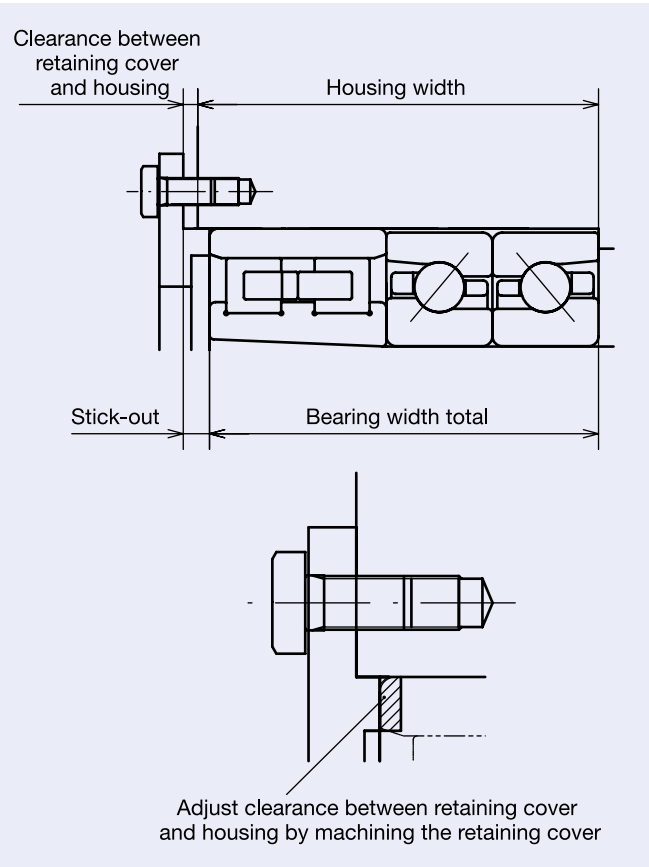
Fig. 1.20 Example of Outer Ring Deformation of a Double-Row Cylindrical Roller Bearing Caused by Tightening Force of Retaining Cover
