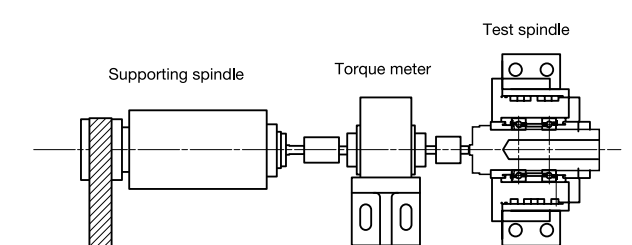
Test Bench Structure
