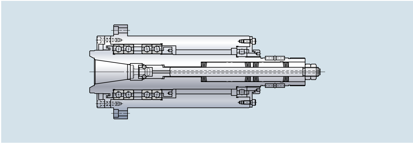
Cutting Spindle
