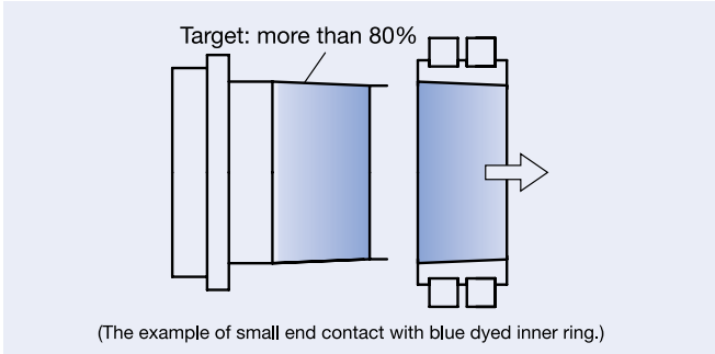
Fig. 1.3 Types of Taper Contact
