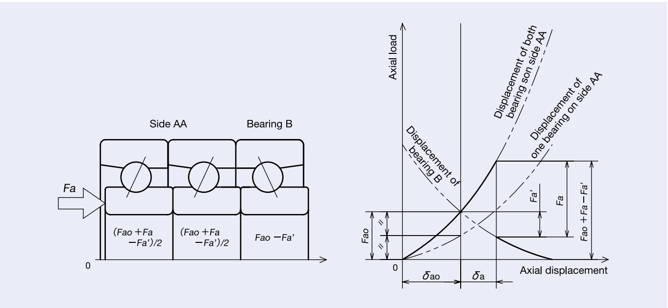
Fig 4.3 Axial Displacement in Position Preload (DBD Arrangement)
