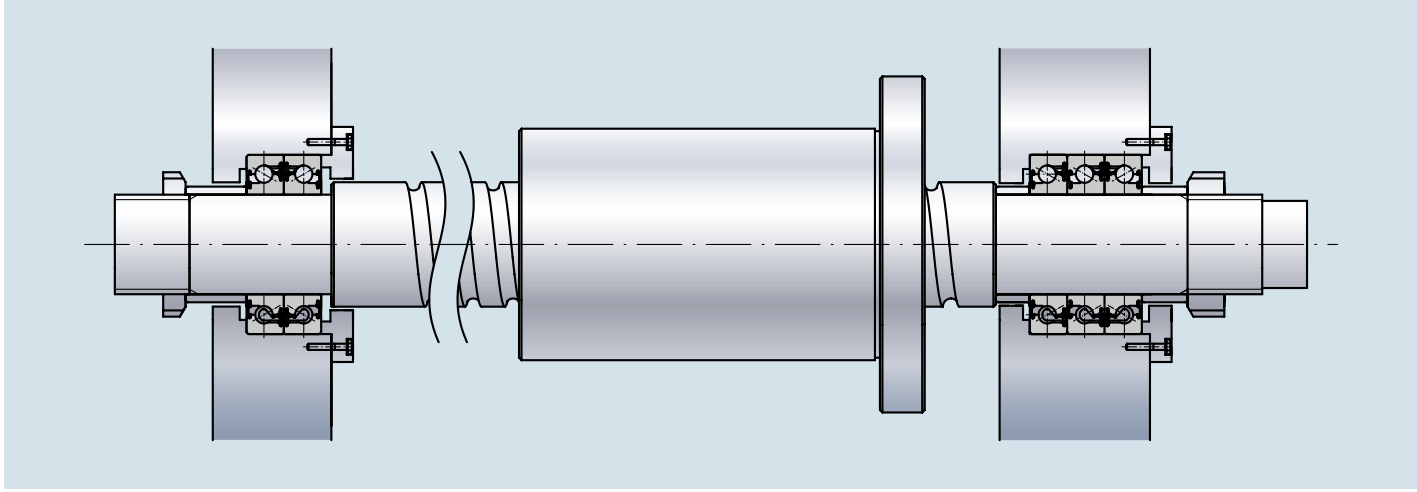
Ball Screw Support
