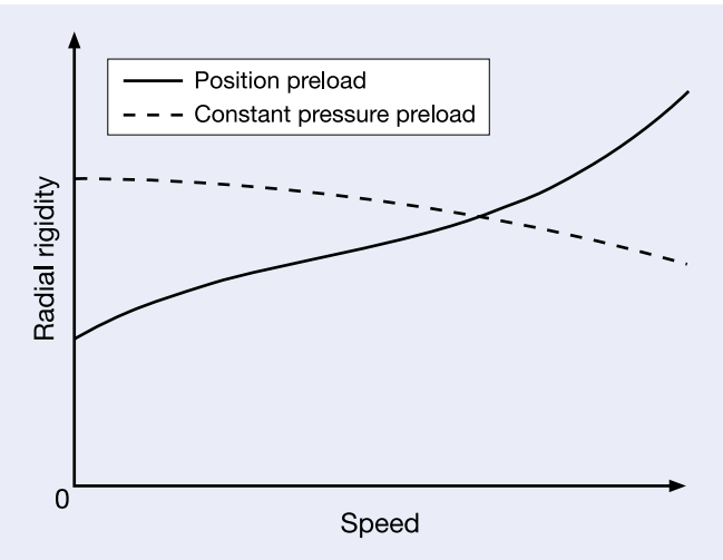
Fig. 4.8 Comparison of Rigidity under each Preloading Method
