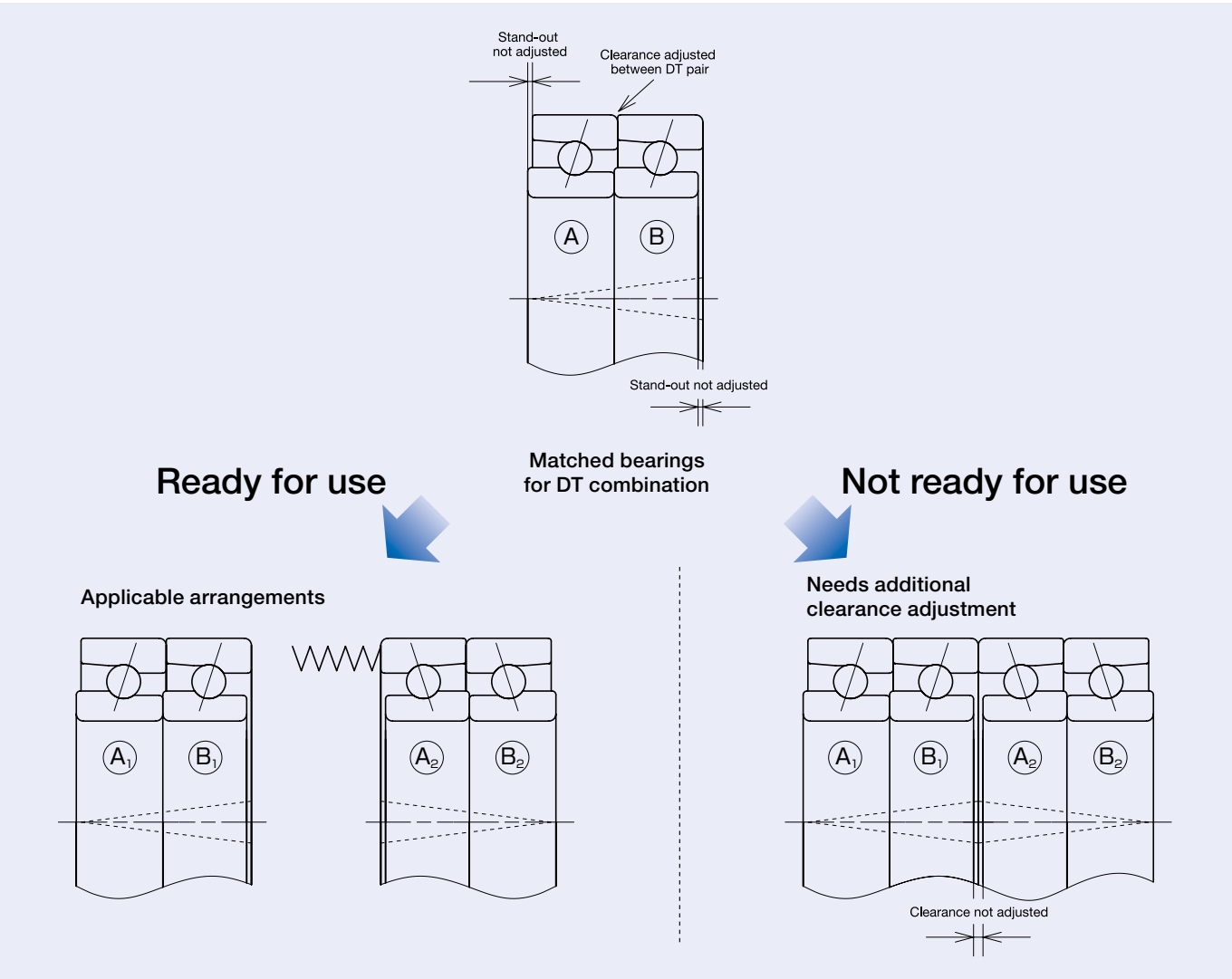
Fig. 3.7 DT Combination
