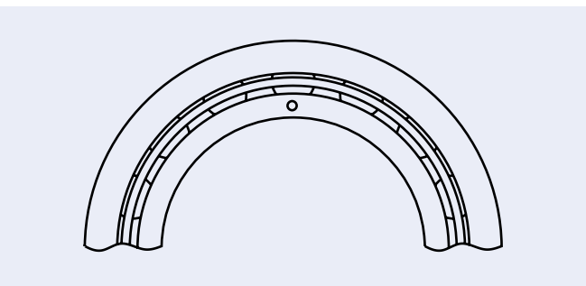
Fig. 3.5 The Symbol for the Position of Maximum Radial Runout of the Inner Ring
