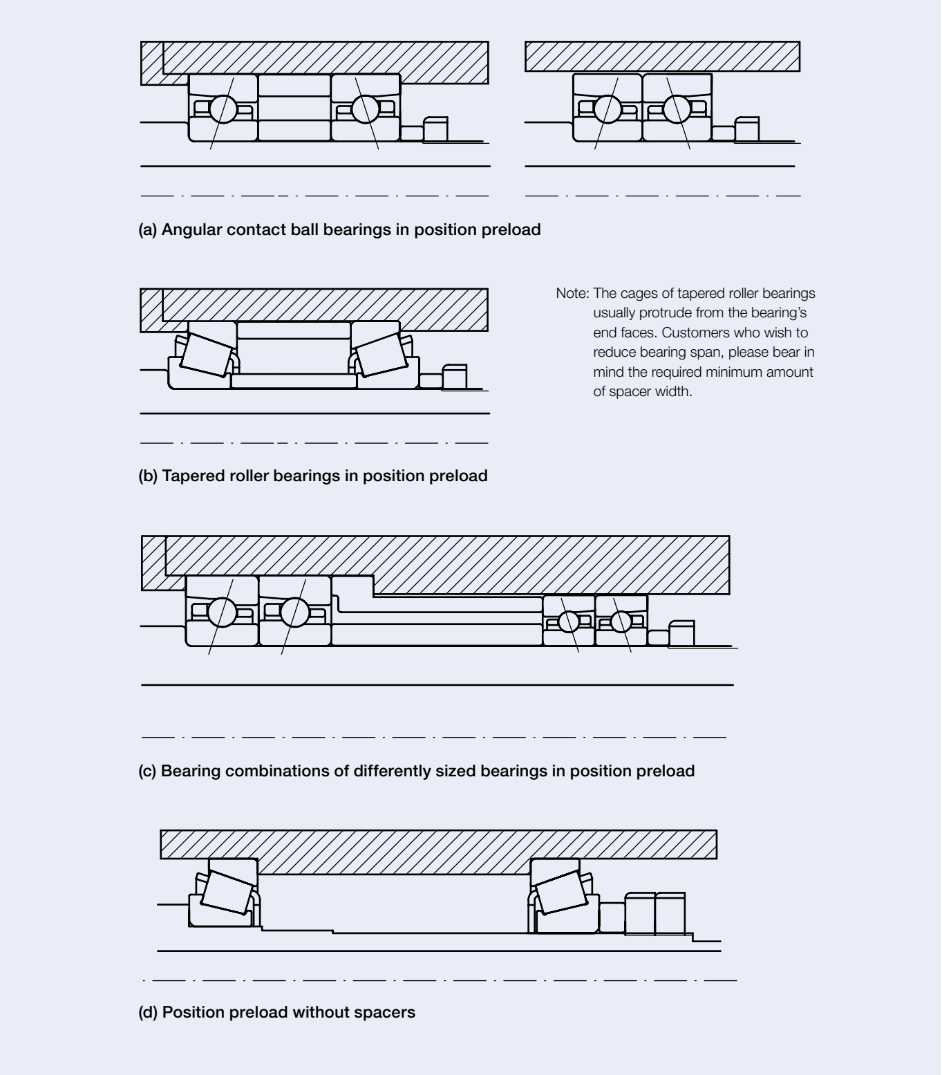
Fig 4.1 Position Preload Examples
