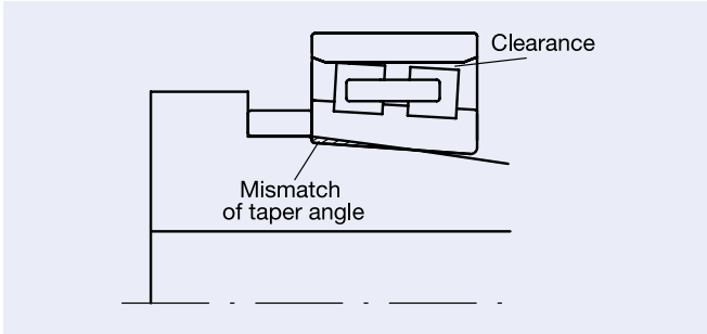
Fig. 1.2 Confirmation of Taper Angle with Coloured Paste
