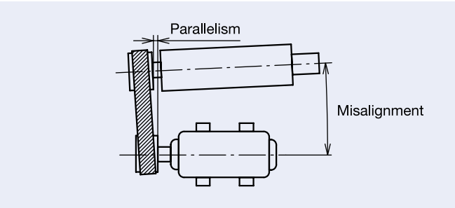
Fig. 2.1 V-belt Drive
