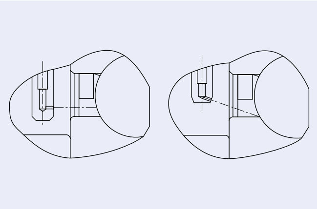
Fig. 9.1 Angle of Spray Nozzle
