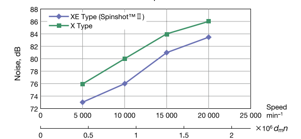
Noise Comparison
