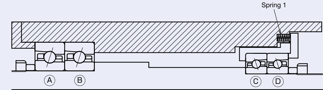
Fig. 4.6 Distribution of Preload in Constant Pressure Preload
