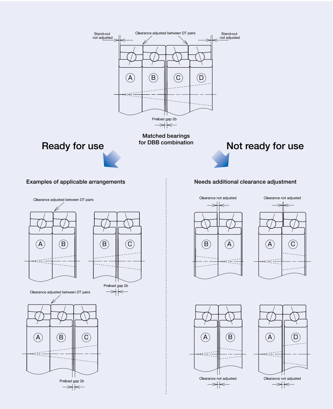
Fig. 3.8 DBB Combination
