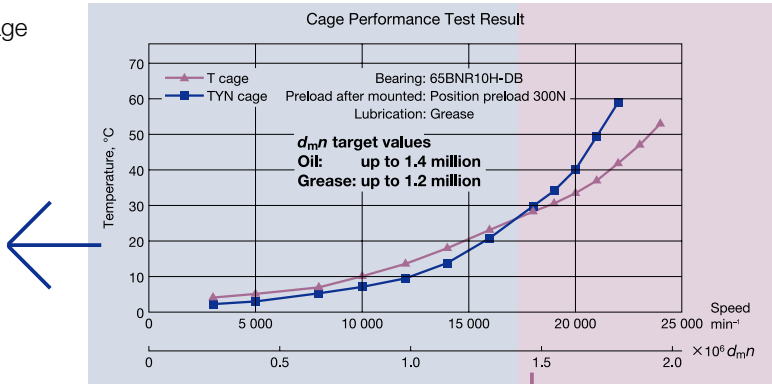
Products: High Accuracy Angular Contact Ball Bearings Standard Series Ultra High Speed Angular Contact Ball Bearings NSKROBUST Series
