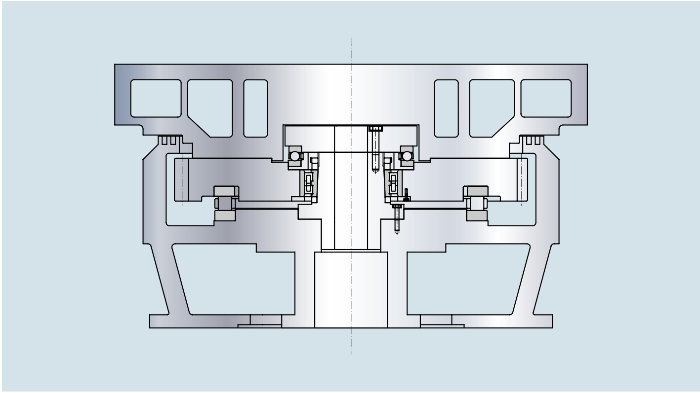
Rotary Table for Vertical Lathe
