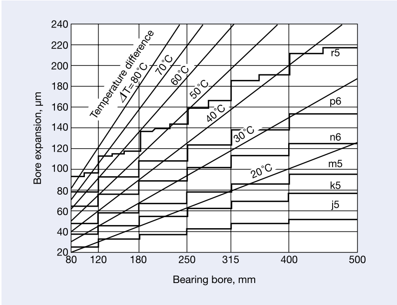
Fig 1.25 Temperature and Thermal Expansion of Inner Ring
