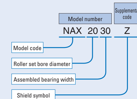
(c) Example of "Bore diameter or roller set bore diameter + width"
