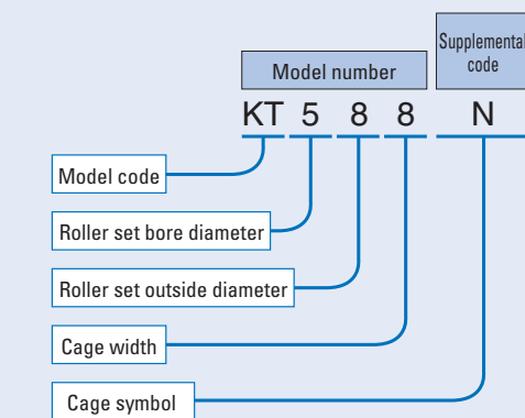
(b) Example of "Bore diameter or roller set bore diameter + Outside diameter or roller set outside diameter + width"
