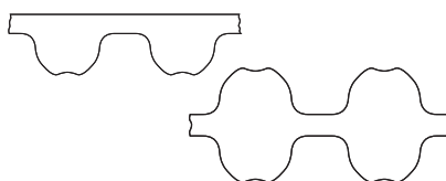
optibelt OMEGA HP / double-sided in cross section
