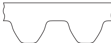
optibelt STD LINEAR in cross section
