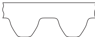
optibelt DELTA Chain in cross section
